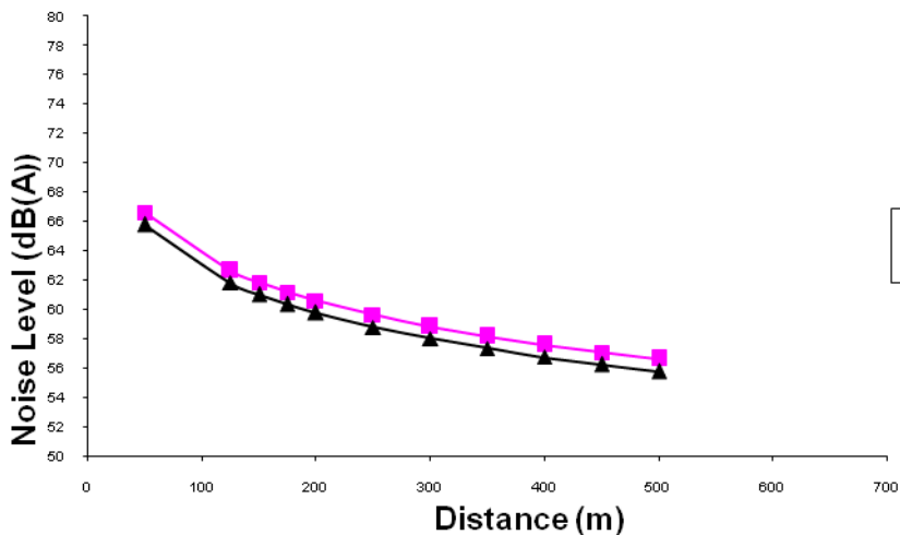
Figure 7.7: Noise Levels, Leq (Day) and Leq (Night) Variation(Madapattu-Thirukovilur Road (SH-9), Year 2040)
