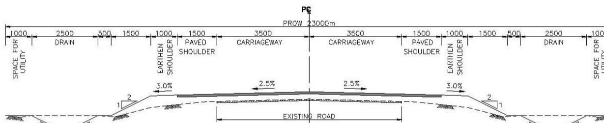
TCS No.2 : 2-LANE RURAL SECTION
