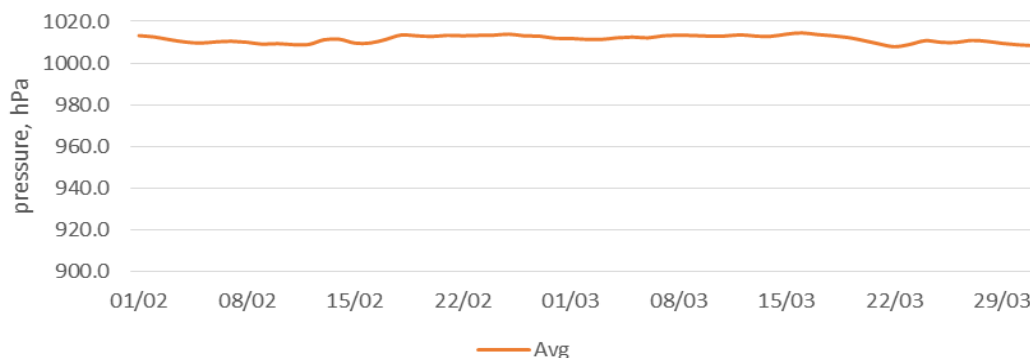
Figure 4.3: Daily variations in Atmospheric Pressure Level
