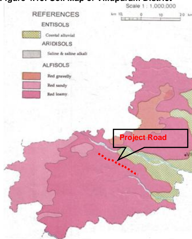
Figure 4.15: Soil Map of Villupuram District
