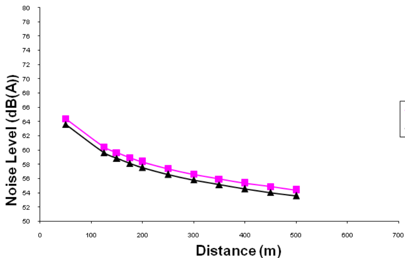
Figure 7.6 : Noise Levels, Leq (Day) and Leq (Night) Variation Madapattu-Thirukovilur Road (SH-9), Year 2030)
