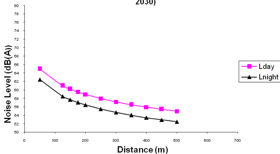
Figure 7.9 : Noise Levels, Leq (Day) and Leq (Night) Variation(Vridhachalam-Parangipettai Road (SH-70), Year 2030)
